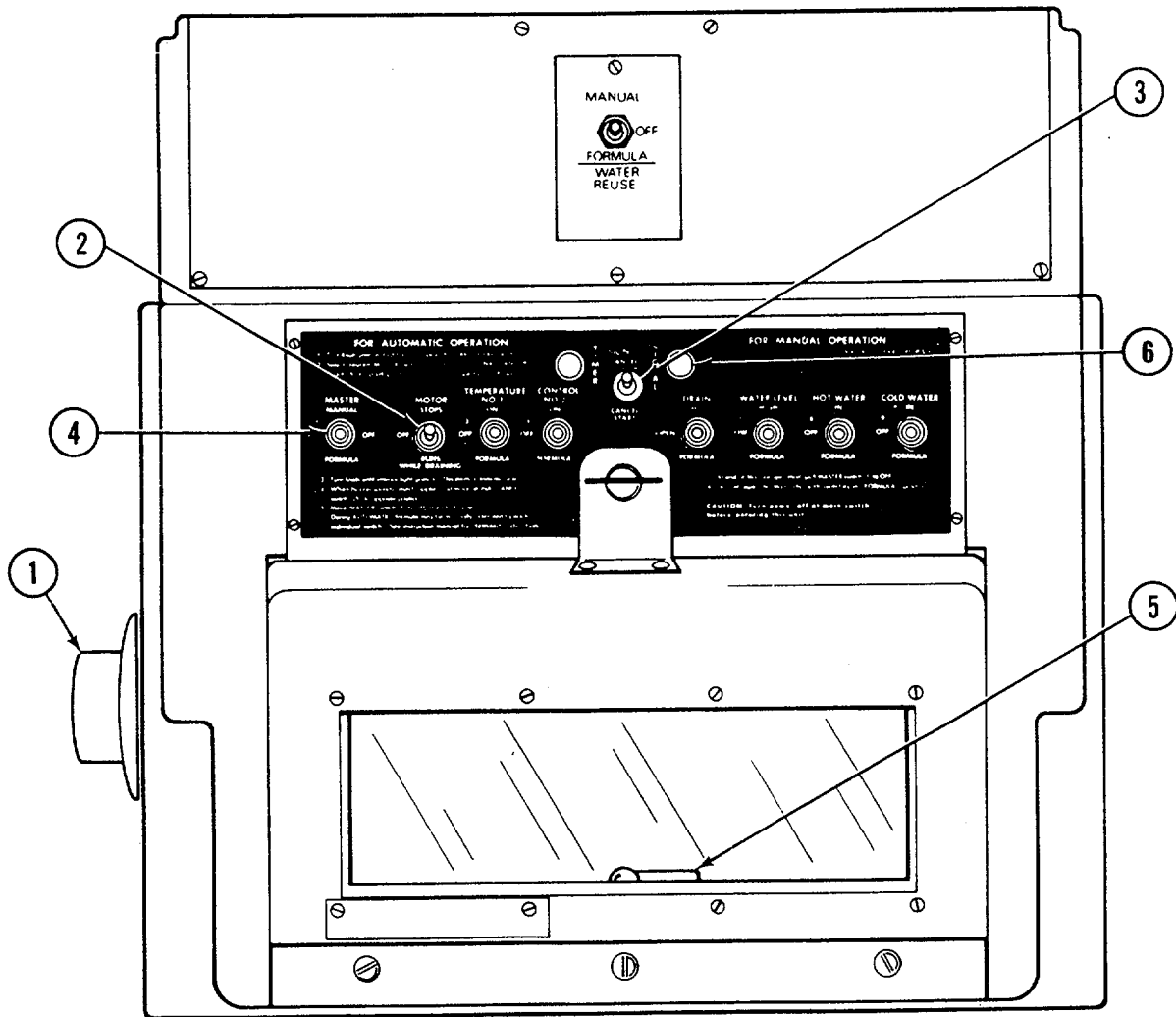
Figure 2-23. Controller .
