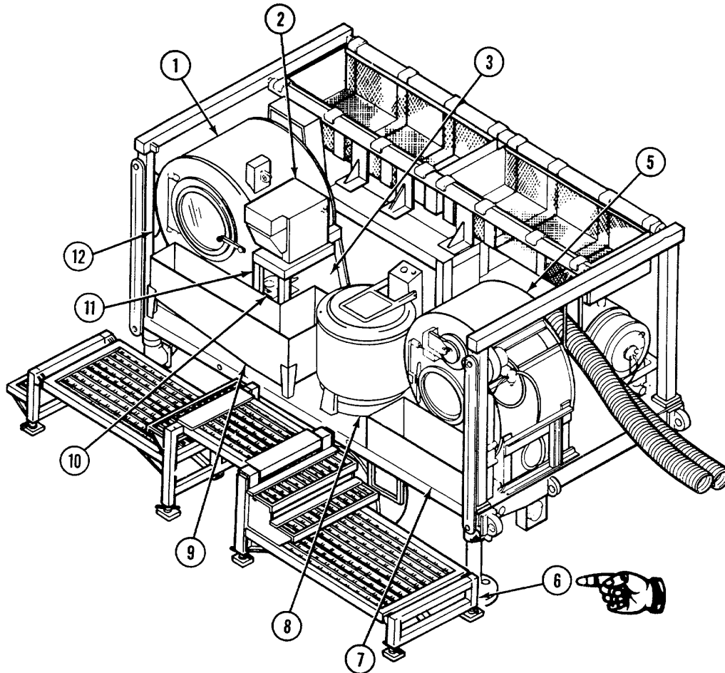
FIGURE 1-1. M85 trailer-mounted laundry unit component location. (Sheet 1 of 2).
